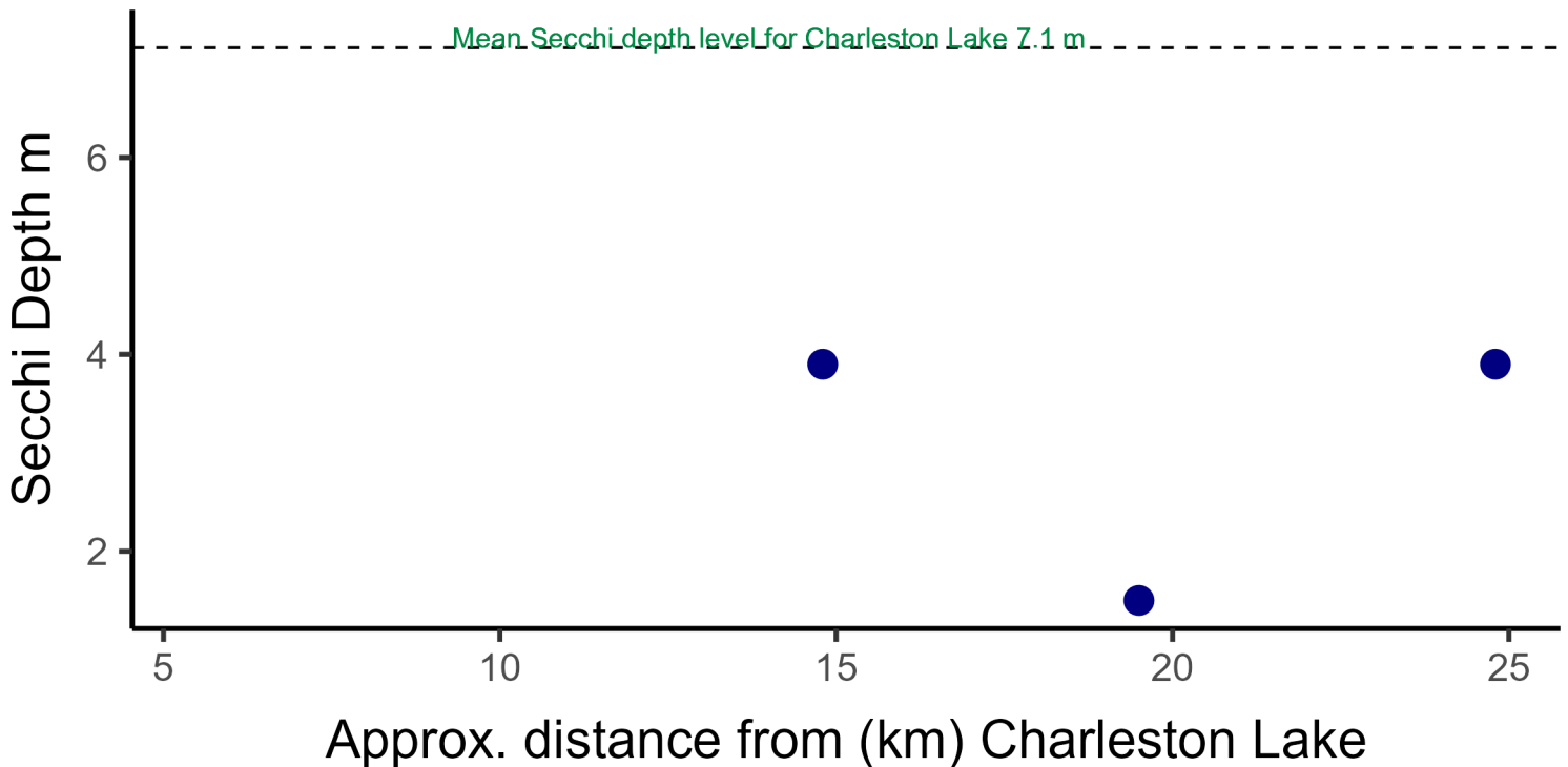
Figure 14. Scatterplot showing 6-year average Secchi depth levels (2018-2023) for lakes sampled within a 25-km radius of Charleston Lake. The dashed line represents Charleston Lake's Secchi depth levels in the LPP since 2018. Lakes with insufficient data were excluded from this analysis. All data were collected by Lake Partner volunteers from 2018-2023.
