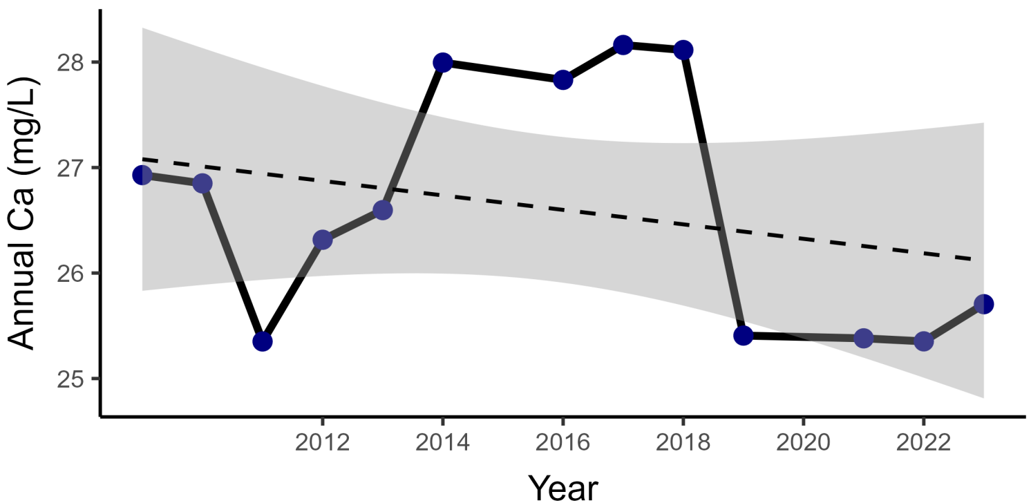
Figure 10. Ca concentrations in Charleston Lake decreased overtime, but this change was not significant. This was determined using a Mann-Kendall trend test, which provided a p-value of 0.6 (a p-value indicates the likelihood of a trend, with a p-value of less than 0.05 providing strong evidence that there is a trend). The shaded area represents the range of values within which we are 95% confident the true calcium concentration is. All samples were taken shortly after the ice-free period of each season. Please note: Ontario’s inland lakes are complex ecosystems, and many factors beyond the indicators monitored by the LPP can affect lake water quality. The trends shown here are meant to provide general information only and may not capture the full complexity of the lake’s water chemistry.
