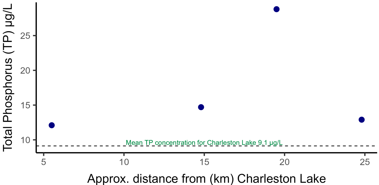
Figure 5. Scatterplot showing 6-year average total phosphorus concentrations (2018-2023) for lakes sampled within a 25-km radius of Charleston Lake. The dashed line represents Charleston Lake's average total phosphorus concentrations in the LPP since 2018. Lakes with insufficient data were excluded from this analysis. All data were collected by Lake Partner volunteers from 2018-2023. Information for each lake within distance of Charleston Lake can be found in the Appendix.
