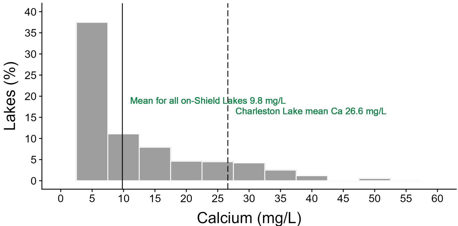
Figure 9. Histogram showing the distribution of ice-free spring average Ca concentrations for 762 lakes located on the Precambrian Shield sampled as part of the Lake Partner Program between the years 2009-2023. The dashed line represents Charleston Lake's spring average ice-free Ca concentration for the years 2009 to 2023 (26.6 mg/L). The solid black line represents the ice-free average calcium concentration of all LPP lakes located off the Precambrian Shield from 2008-2023 ( 9.8 mg/L). The level at which some aquatic animals (mainly, some Daphnia ) become at risk of Ca deficiency is 1.5 mg/L.
