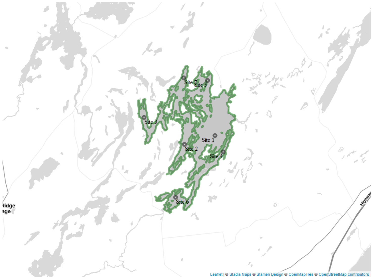
Figure 1. A map showing Charleston Lake and the location of the Lake Partner Program sampling sites. Past six year averages of the parameters for each site can be found in Appendix A. Sites with insufficient data were excluded from this analysis. All data were collected by Lake Partner volunteers from 2018-2023.
