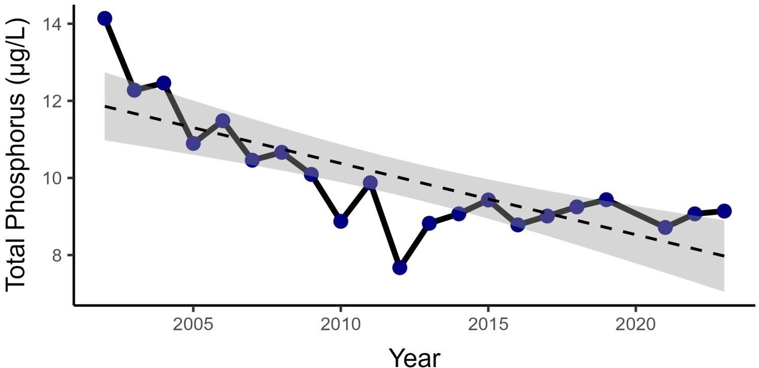
Figure 4. In general, the overall trend in TP concentrations of Charleston Lake have decreased overtime, this change was significant. This was determined using a Mann-Kendall trend test, which provided a p-value of 0.000411 (a p-value indicates the likelihood of a trend, with a p-value of less than 0.05 providing strong evidence that there is a trend). The blue points represent the average ice-free spring TP concentration for each year. The dotted line represents a linear model representing the overall trend over time. The shaded area represents the range of values within which we are 95% confident the true TP concentration lies. Please note: Ontario's inland lakes are complex ecosystems, and many factors beyond the indicators monitored by the Lake Partner Program can affect lake water quality. The trends shown here are meant to provide general information only and may not capture the full complexity of the lake's water chemistry.
