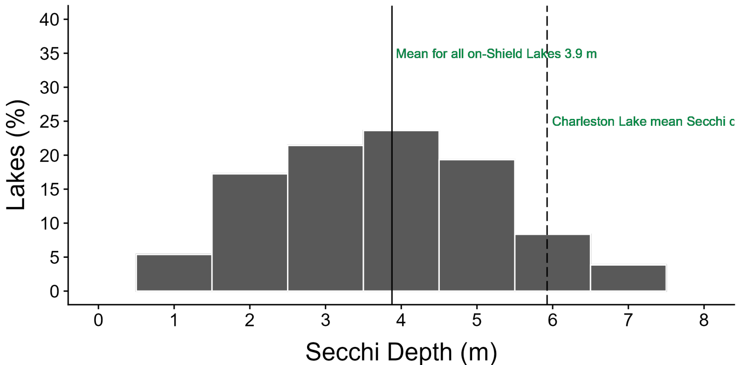
Figure 12. Histogram showing the distribution of Secchi depths (measured with a Secchi disk, Secchi depth is used as a representative of water clarity) for 923 LPP lakes for years 1996-2023. The dashed line represents the mean Secchi depth (5.9) (m) for Charleston Lake. The solid line represents the average Secchi depth of all LPP lakes located on the Precambrian Shield (3.9). Note that Secchi depth averages for each lake were calculated using data collected in July-September, as previous research has shown that these are the most stable months for inland lake water clarity and hence, are suitable for making comparisons among lakes (MECP, unpublished data; Bruhn & Soranno (2005)).
