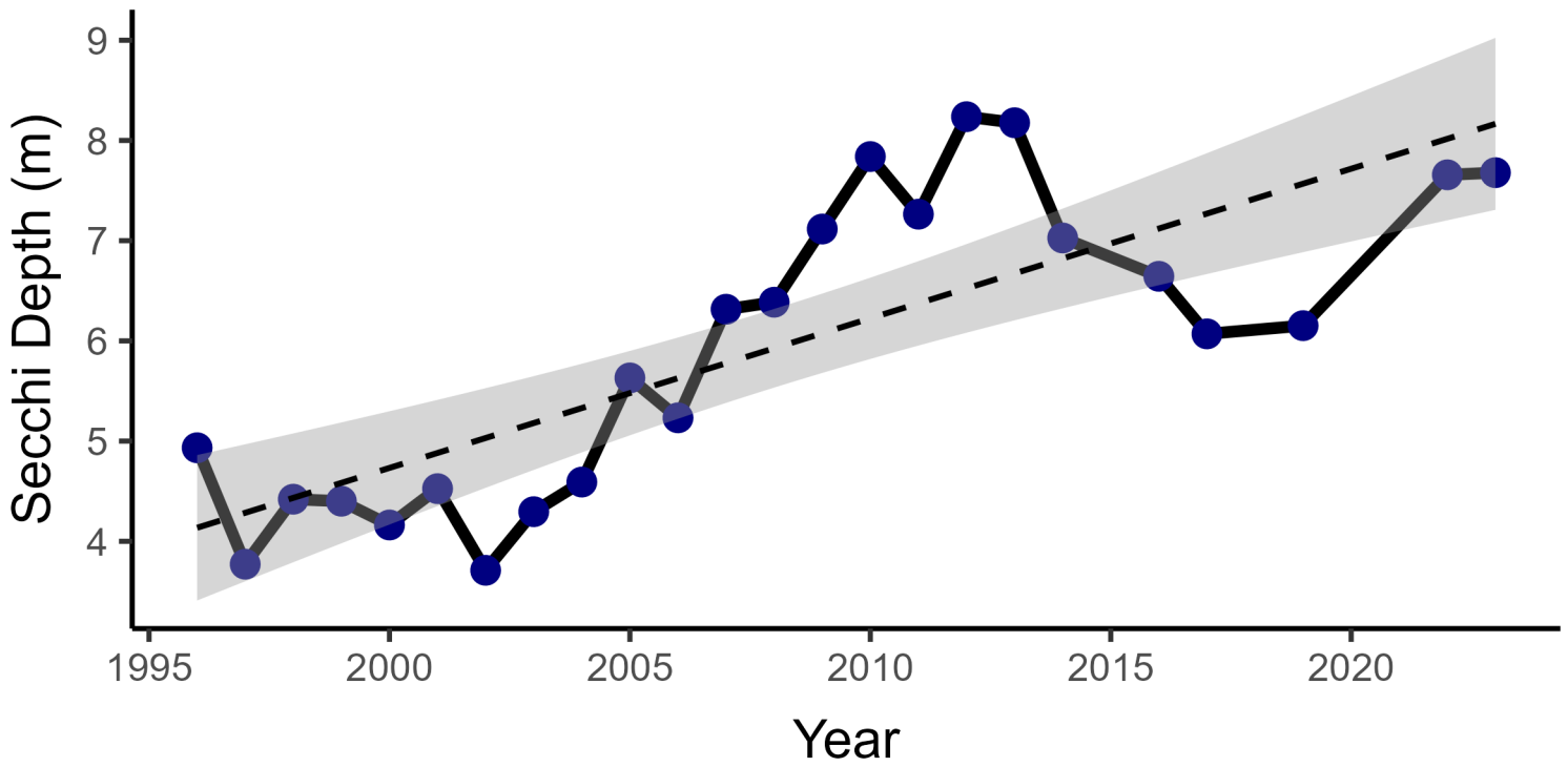
Figure 13. Water clarity (as measured with a Secchi disk) in Charleston Lake have increased over time, this change was significant. This was determined using a Mann-Kendall trend test, which provided a p-value of 0.0 (a p-value indicates the likelihood of a trend, with a p-value of less than 0.05 providing strong evidence that there is a trend). The blue points represent the average Secchi depths for July-September of each year. The dotted line represents a linear model representing the overall trend over time. The shaded area represents the range of values within which we are 95% confident the true Secchi depth lies. Please note: Ontario’s inland lakes are complex ecosystems, and many factors beyond the indicators monitored by the LPP can affect lake health. All samples taken during ice-free season of each year (May-October). Please note: Ontario’s inland lakes are complex ecosystems, and many factors beyond the indicators monitored by the LPP can affect lake water quality. The trends shown here are meant to provide general information only and may not capture the full complexity of the lake’s water chemistry.
