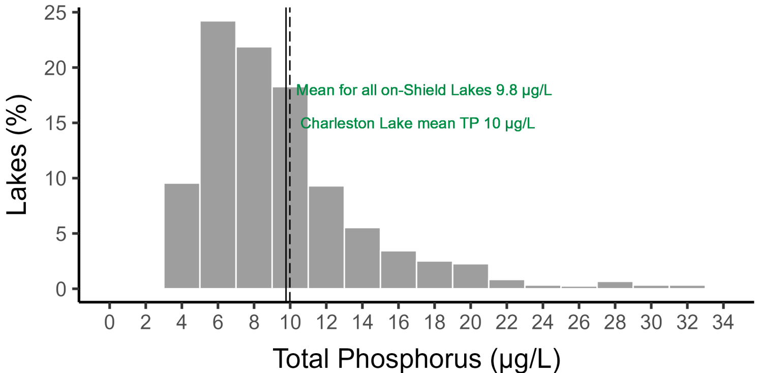
Figure 3. Histogram showing the distribution of average ice-free TP concentrations for 1200 lakes located on the Precambrian Shield, sampled as part of the Lake Partner Program between the years 2002-2023. The dashed line represents Charleston Lake's spring average TP concentration for the years 2002-2023 ( 10.0 \mu\text{g/L} ). The solid black line represents the ice-free spring average TP concentration of all LPP lakes located on the Precambrian Shield from 2002-2023 ( 9.8 \mu\text{g/L} ). Most lakes are less than the Provincial Water Quality Objective of 20 \mu\text{g/L} .
