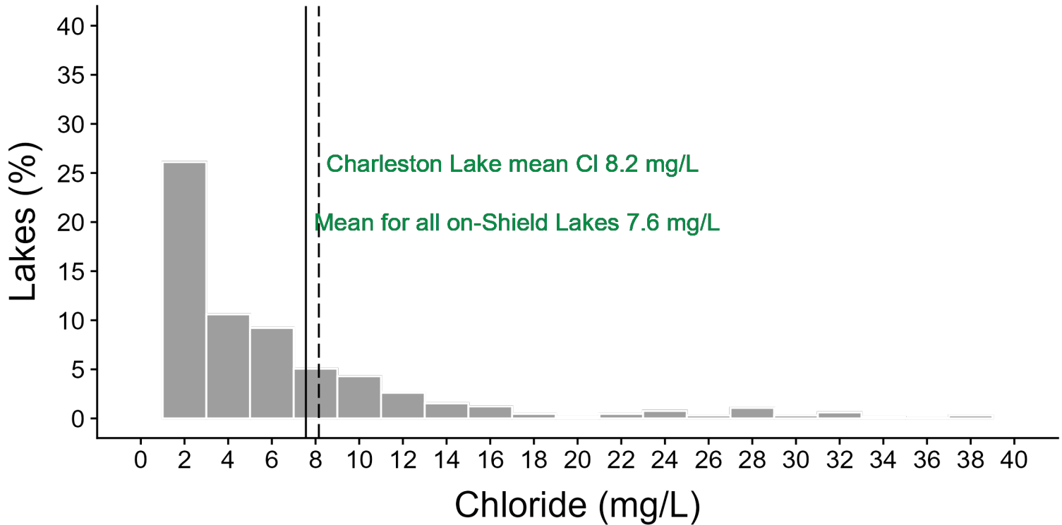
Figure 6. Histogram showing the distribution of ice-free spring average Cl concentrations for 675 lakes located on the Precambrian Shield sampled as part of the Lake Partner Program between the years 2016-2023. The dashed line represents Charleston Lake's spring average ice-free Cl concentration for the years 2016 to 2023 (8.2 mg/L). The solid black line represents the ice-free average Cl concentrations of all LPP lakes located off the Precambrian Shield (7.6 mg/L). All lakes in this data set fall below the Canadian Water Quality Guideline for the Protection of Aquatic Life of 120 mg/L Cl.
