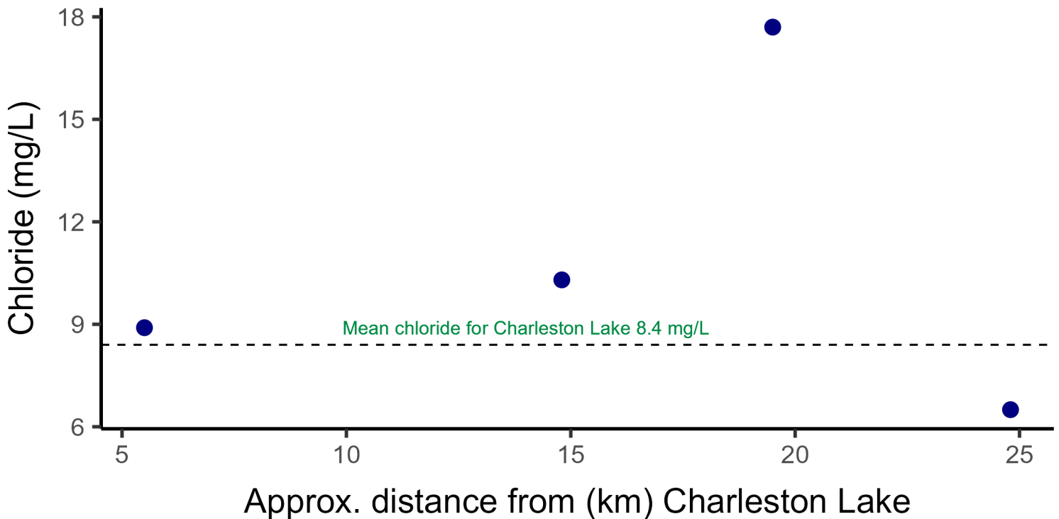
Figure 8. Scatterplot showing 6-year average chloride concentrations (2018-2023) for lakes sampled within a 25-km radius of Charleston Lake. The dashed line represents Charleston Lake's average chloride concentrations in the LPP since 2018. Lakes with insufficient data were excluded from this analysis. All data were collected by Lake Partner volunteers from 2018-2023. Information for each lake within distance of Charleston Lake can be found in the Appendix.
