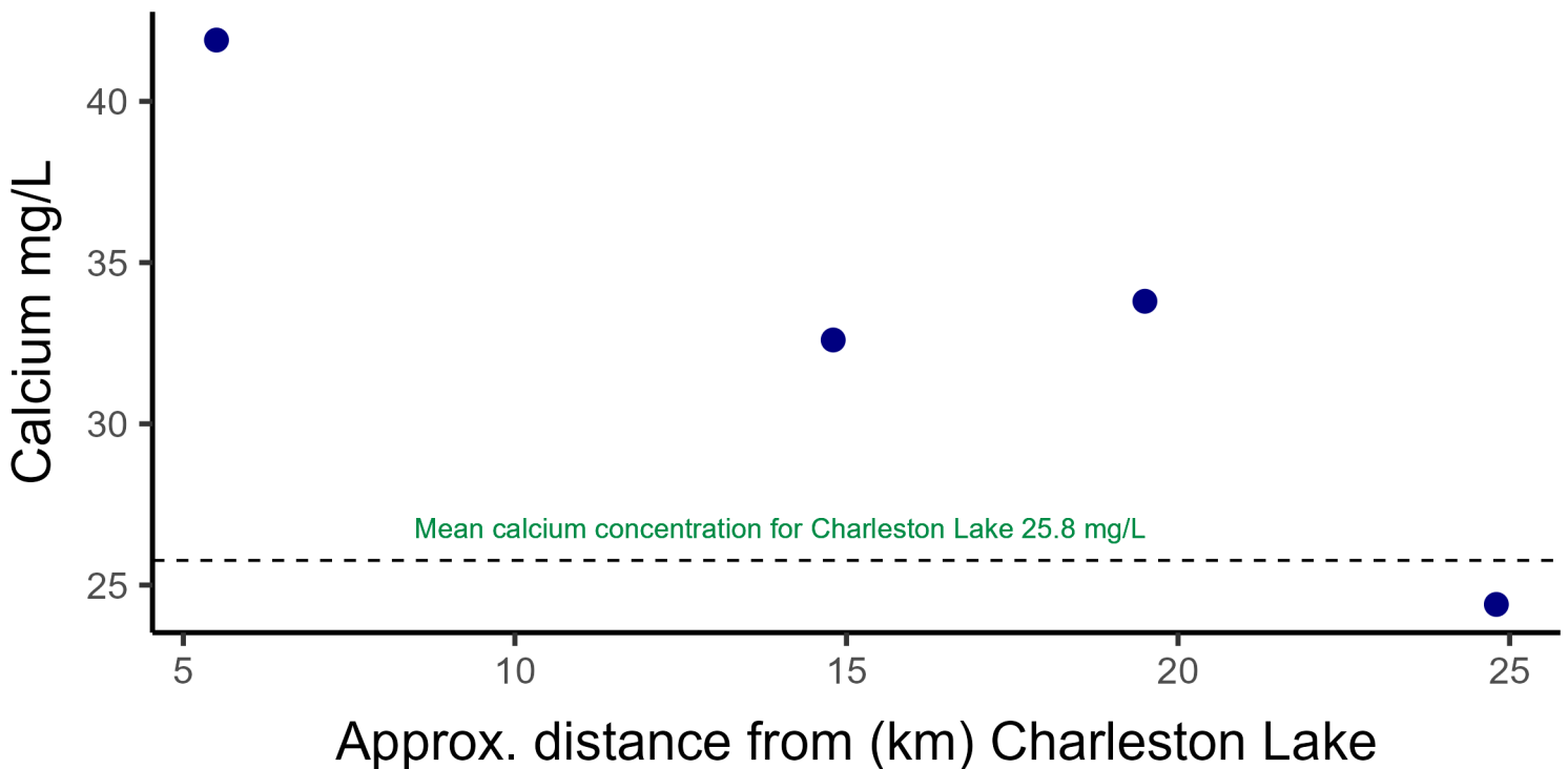
Figure 11. Scatterplot showing 6-year average calcium concentrations (2018-2023) for lakes sampled within a 25-km radius of Charleston Lake. The dashed line represents Charleston Lake's average calcium concentrations in the LPP since 2018. Lakes with insufficient data were excluded from this analysis. All data were collected by Lake Partner volunteers from 2018-2023.
