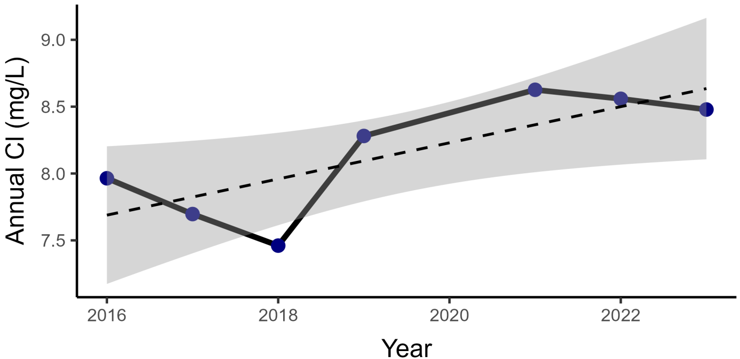
Figure 7. Cl concentrations in Charleston Lake increased overtime , but this change was not significant. This was determined using a Mann-Kendall trend test, which provided a p-value of 0.2 (a p-value indicates the likelihood of a trend, with a p-value of less than 0.05 providing strong evidence that there is a trend). The shaded area represents the range of values within which we are 95% confident the true chloride concentration is. All samples were taken shortly after ice-off of each season. Please note: Ontario’s inland lakes are complex ecosystems, and many factors beyond the indicators monitored by the LPP can affect lake water quality. The trends shown here are meant to provide general information only and may not capture the full complexity of the lake’s water chemistry.
